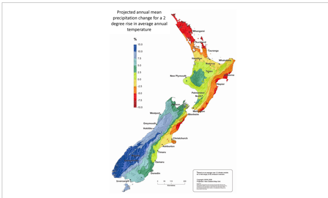
Figure 1: Projected New Zealand Climate change impacts
