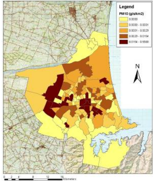
Figure A2-27. CAU map displaying industrial PM 10 emissions between 10pm and 6am for a typical winters day in 1999
