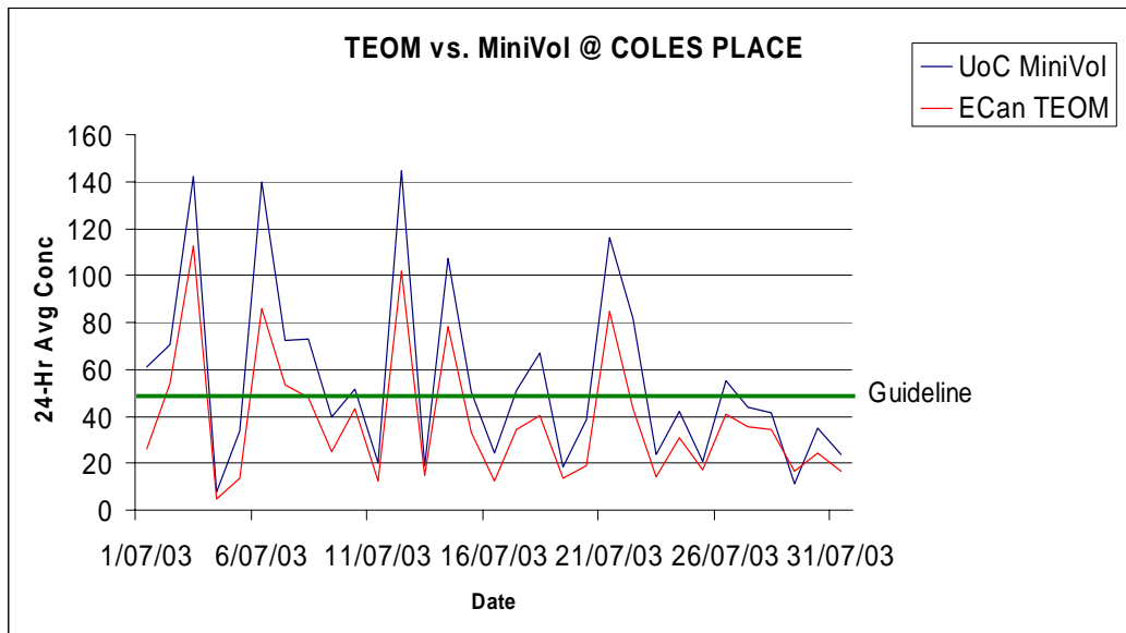
Figure A2-50. Comparison of daily averages from the TEOM and MiniVol. St Albans (Coles Place), July 2003.
