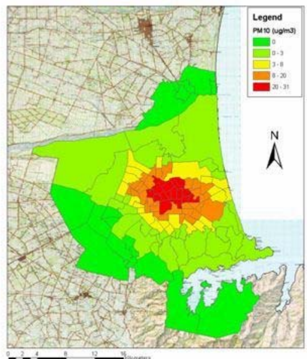
Figure A2-70. Annual PM 10 census area unit exposure map. Dark CAUs represent areas with values above the 20 µg m -3 Ministry for the Environment guideline.
