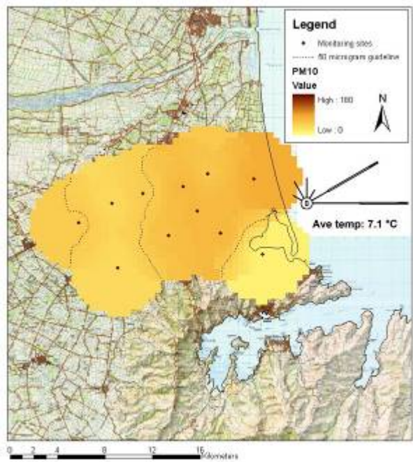
Figure A2-57. 500m grid displaying 24hr average PM 10 in \mu\text{gm}^{-3} for 2 nd – 3 rd July 2003
