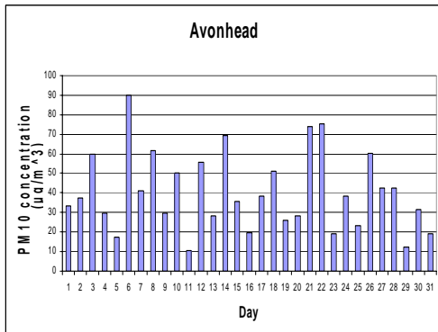
Figure A2-47. Oaklands, Hornby and Avonhead. Daily PM 10 averages for the month of July 2003
