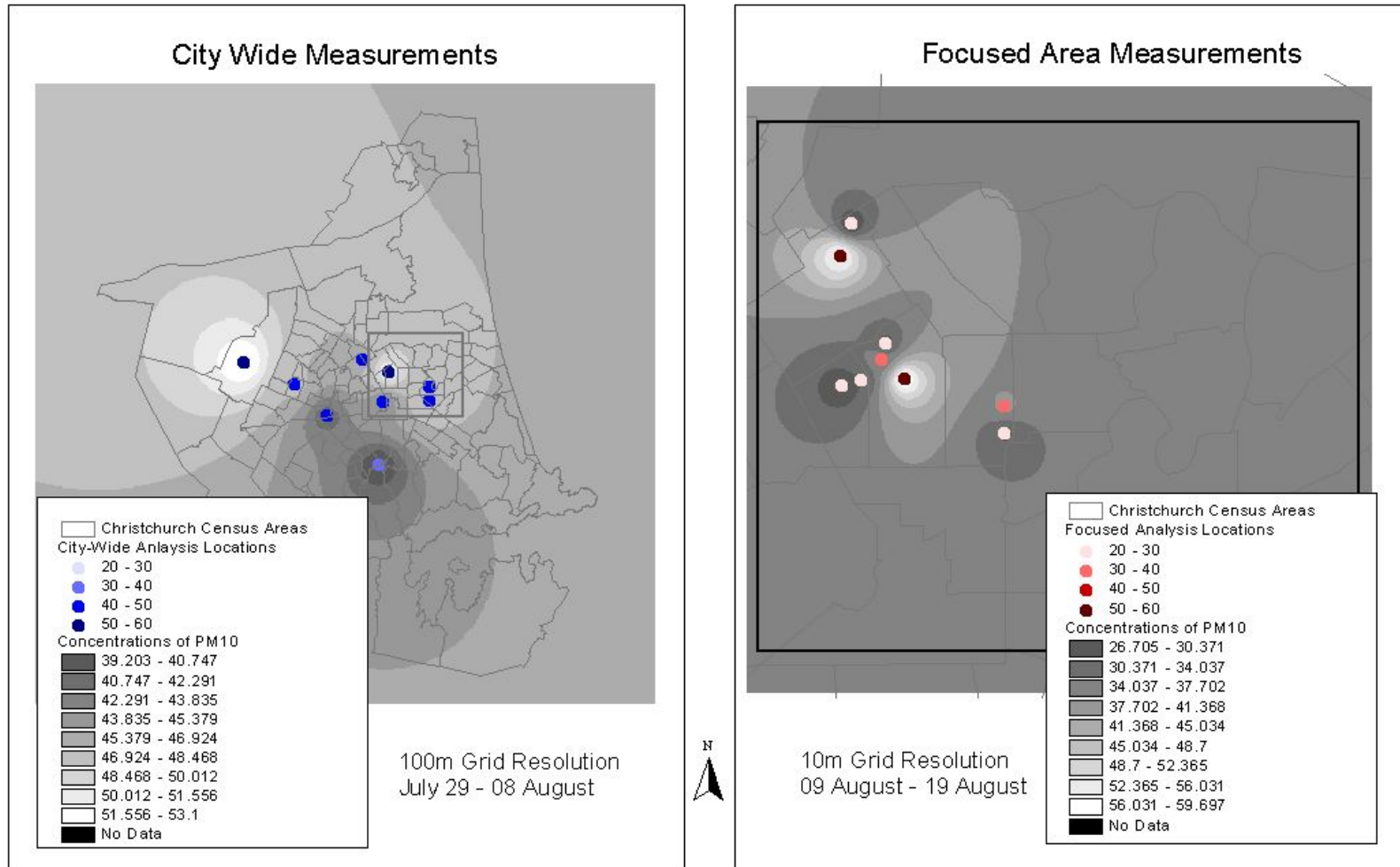
Figure A2-42. Spatial patterns in PM 10 , Christchurch 2002
