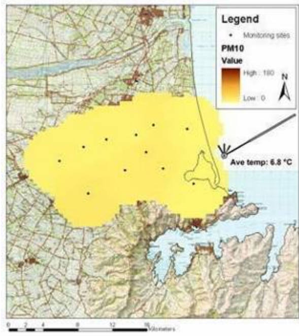
Figure A2-59. 500m grid displaying 24hr average PM 10 in \mu\text{gm}^{-3} for 29 th – 30 th July 2003
