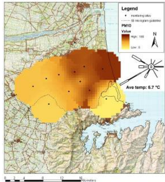
Figure A2-54. 500m grid displaying 24hr average PM 10 in \mu\text{g m}^{-3} for 3 rd – 4 th July 2003.
