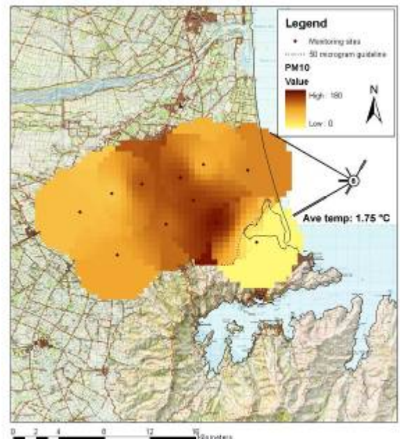
Figure A2-55. 500m grid displaying 24hr average PM 10 in \mu\text{g m}^{-3} for 12 th – 13 th July 2003
