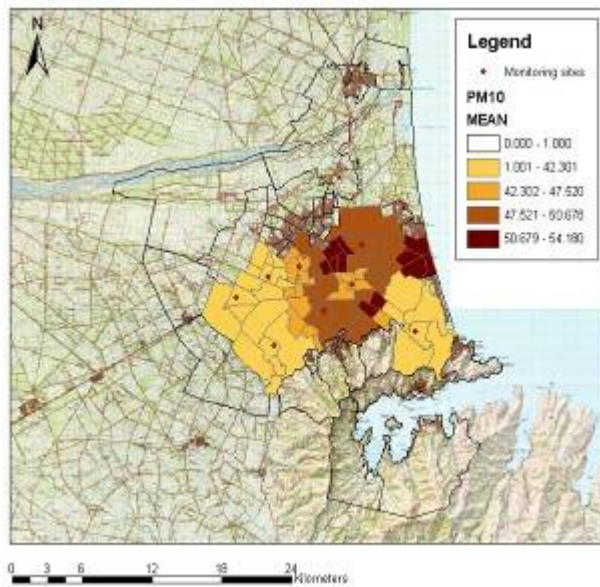
Figure A2-53. Census area unit map displaying monthly average PM 10 in \mu\text{g m}^{-3} for July 2003 derived from interpolated monitoring data
