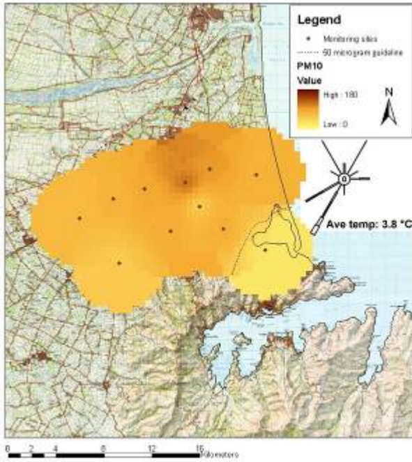
Figure A2-56. 500m grid displaying 24hr average PM 10 in \mu\text{gm}^{-3} for 21 st – 22 nd July 2003
