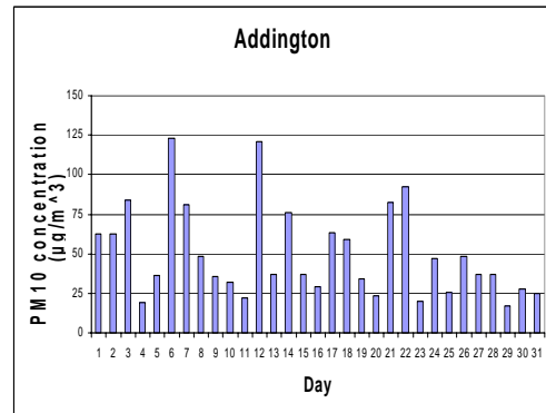
Figure A2-46. Woolston, Mt. Pleasant and Addington. Daily PM 10 averages for the month of July 2003
