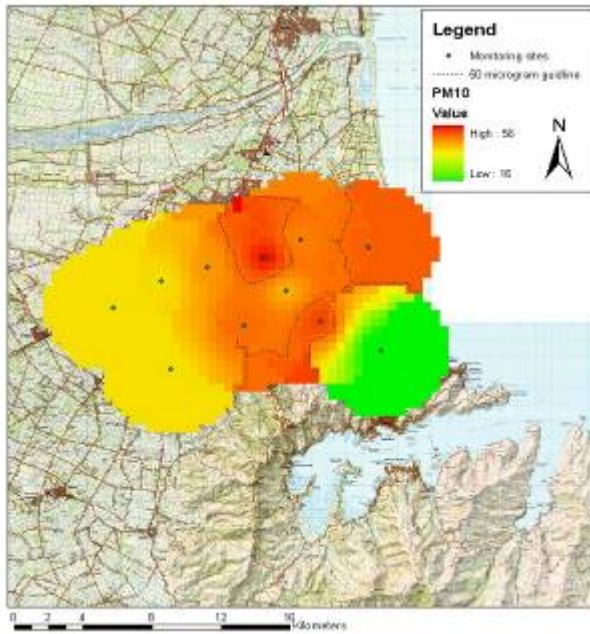
Figure A2-52. 500m grid displaying monthly average PM 10 in \mu\text{g m}^{-3} for July 2003
