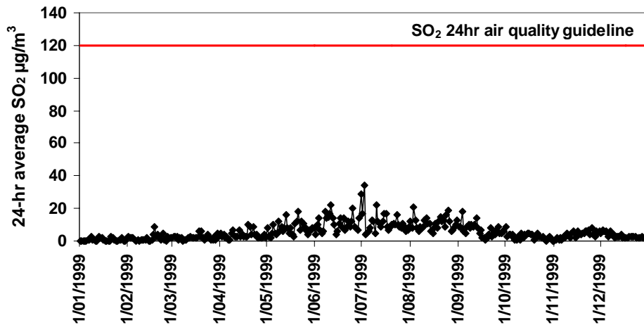
Figure A2-78. SO 2 24-hour average during 1999 measured at Packe Street St Albans.
