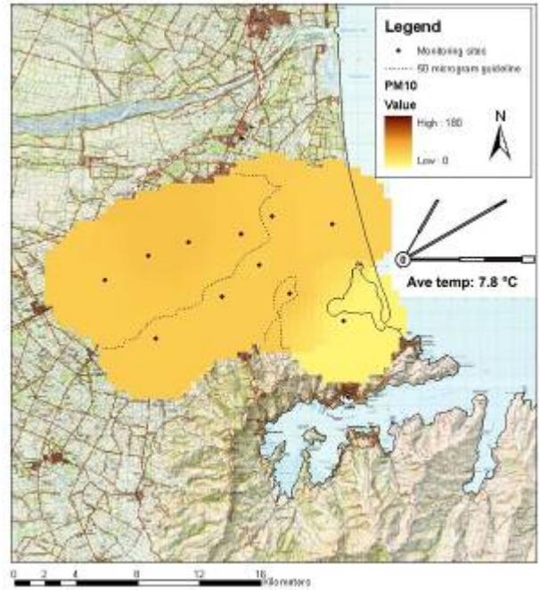
Figure A2-58. 500m grid displaying 24hr average PM 10 in \mu\text{gm}^{-3} for 26 th – 27 th July 2003
