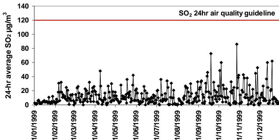
Figure A2-79. SO 2 24-hour average during 1999 measured at Hornby.
