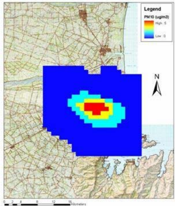
Figure A2-69. Annual vehicle PM 10 exposure grid from TAPM.
