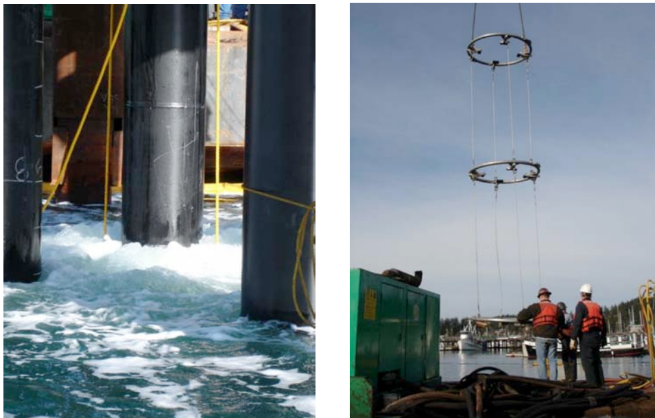
Figure 3.1: Bubble Net Curtain Air Release Rings (left) and in use (right)
