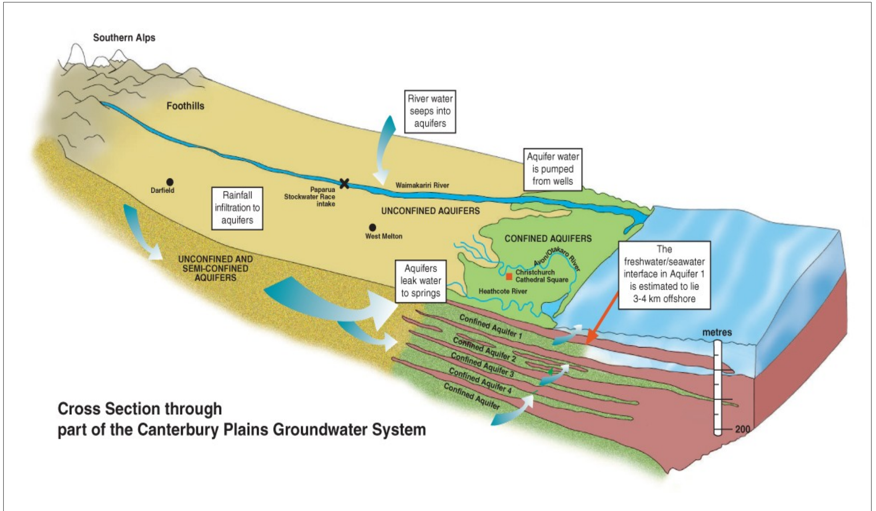
Figure 1: Cross section showing the aquifers of the Christchurch Groundwater System
