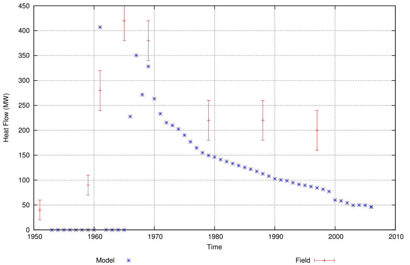
Fig. 3.12: Surface heat flow at Karapiti
