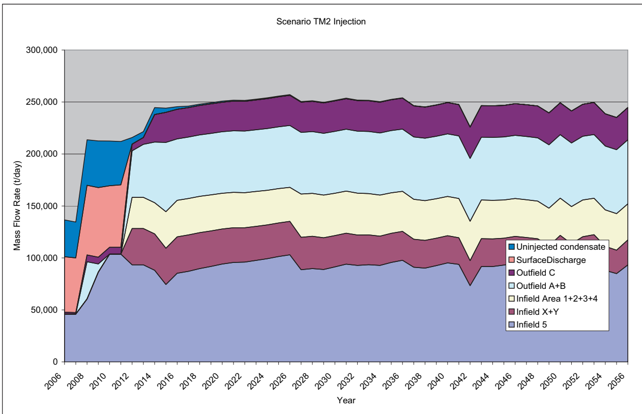
Fig. 4.18: Injection: TM 2
